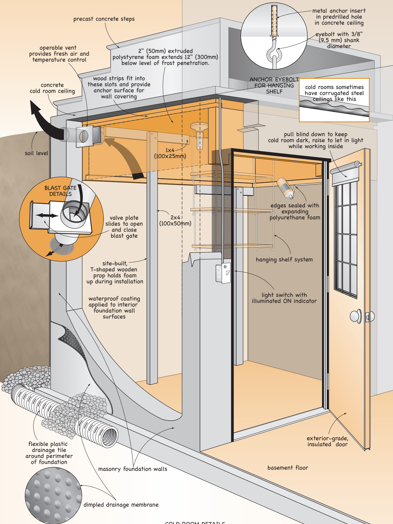
COLD ROOM DETAILS
