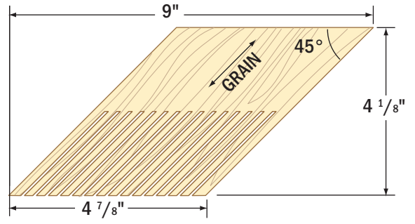
FEATHER BOARD DETAIL
