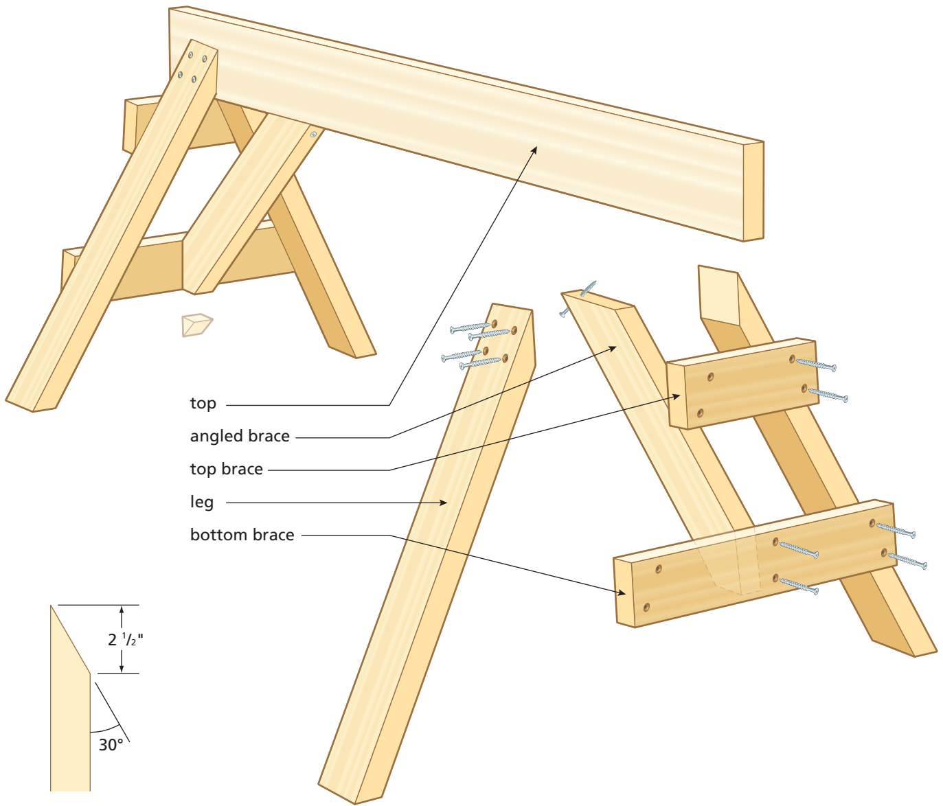
LEG TOP ANGLE DETAIL
