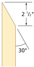
LEG TOP ANGLE DETAIL
